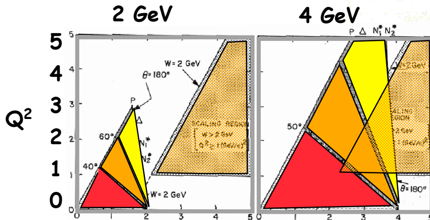
\nu - Electron energy loss (GeV)
